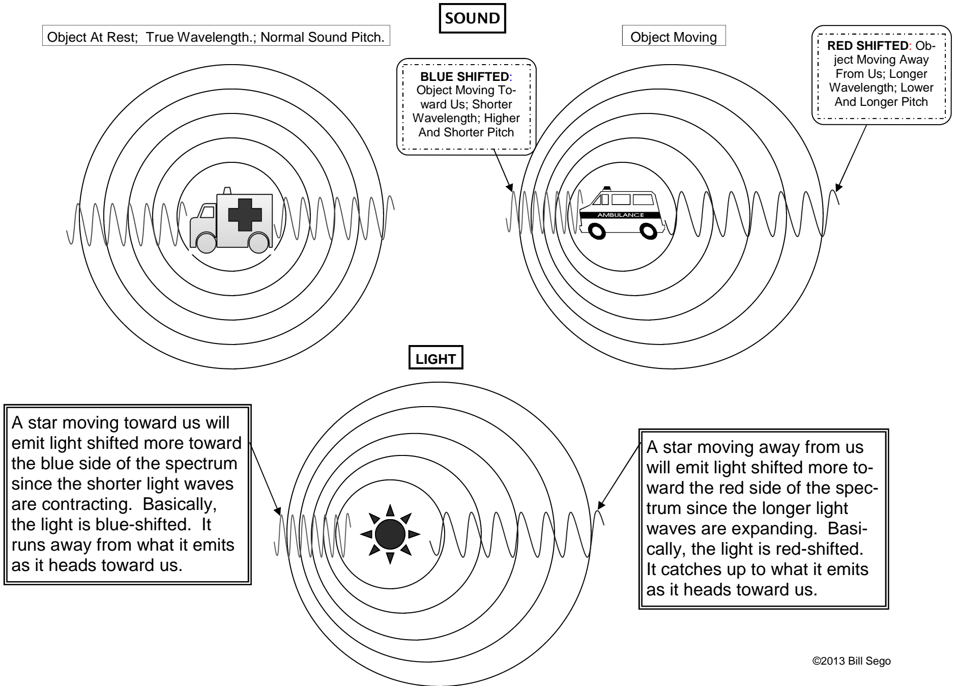
Figure 8.1: THE DOPPLER EFFECT
