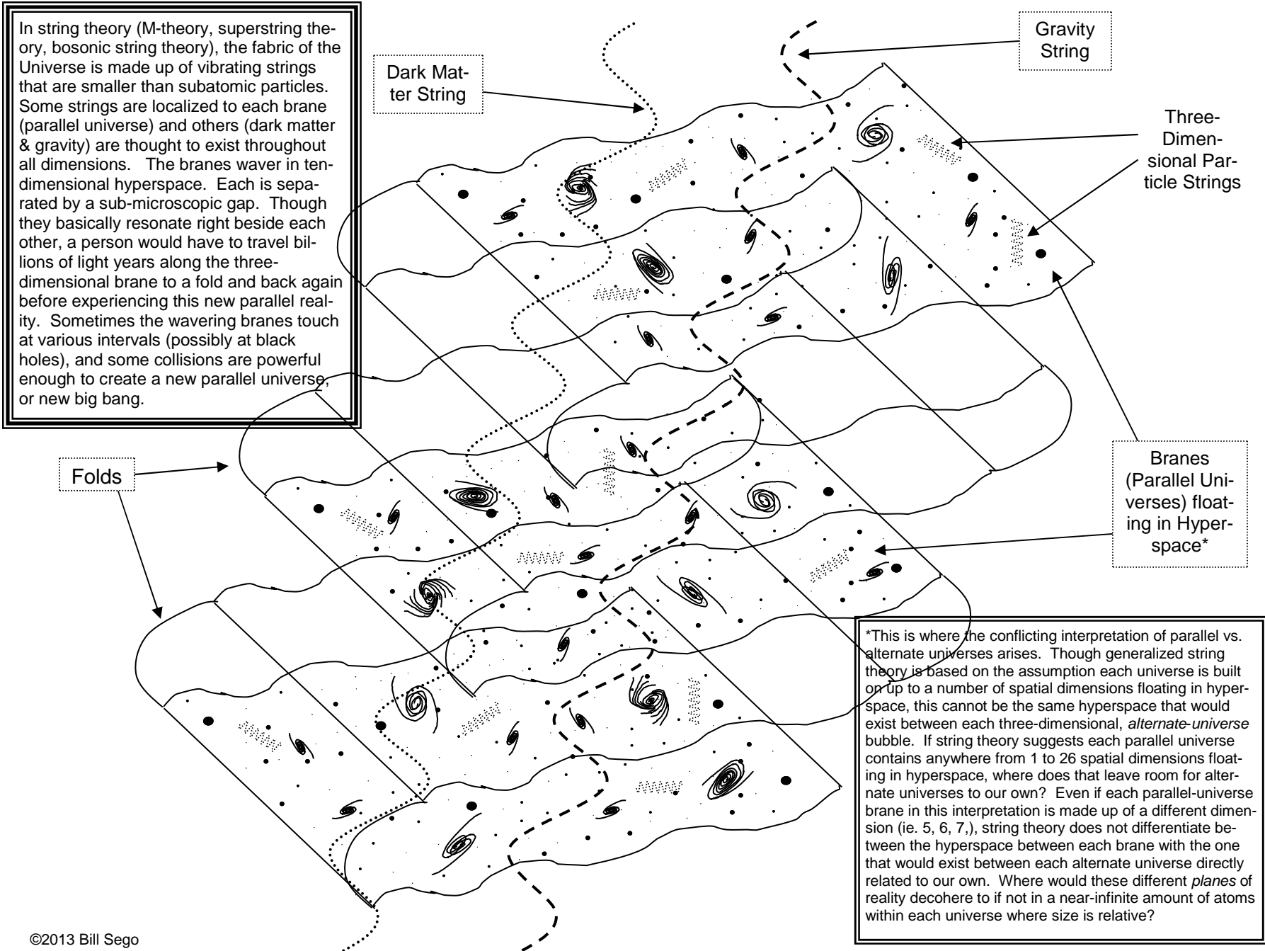
Figure 4.3: STRING THEORY & MULTIPLE DIMENSIONS
