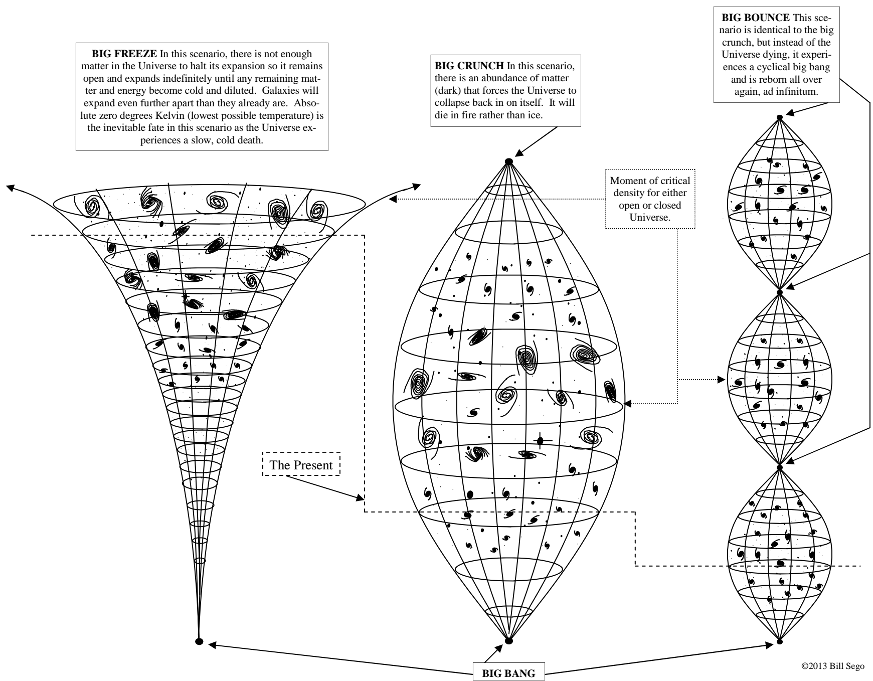
Figure 13.1: BIG CRUNCH / BIG FREEZE / BIG BOUNCE
