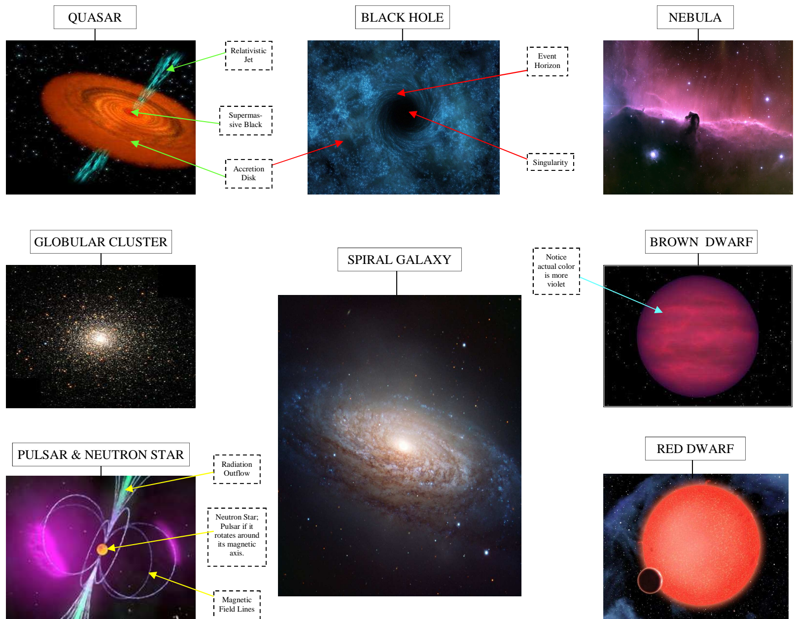
Figure 1.3: UNIVERSE STRUCTURES
