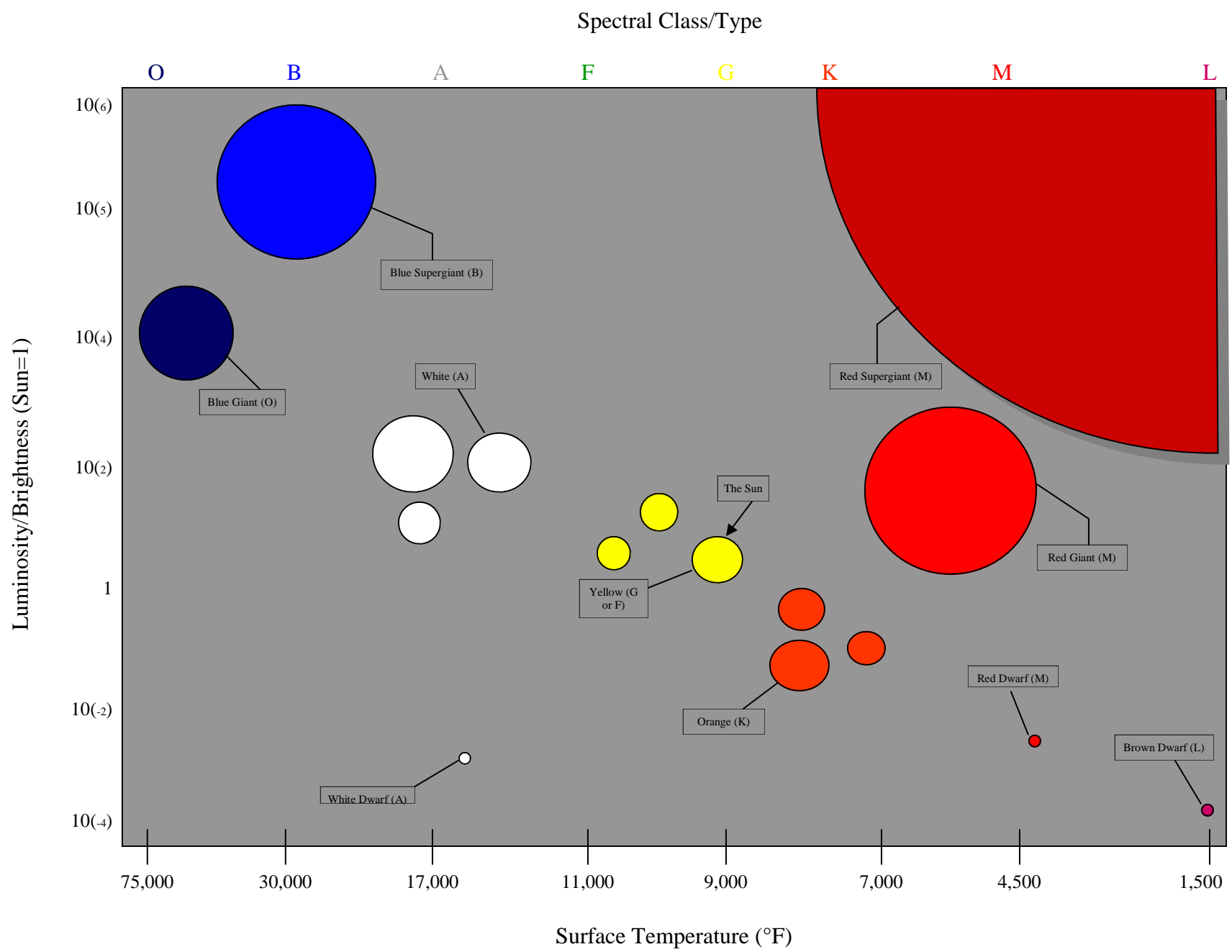
Figure 1.2: STAR COLOR AND TYPE (Based on Hertzsprung-Russell Diagram)
