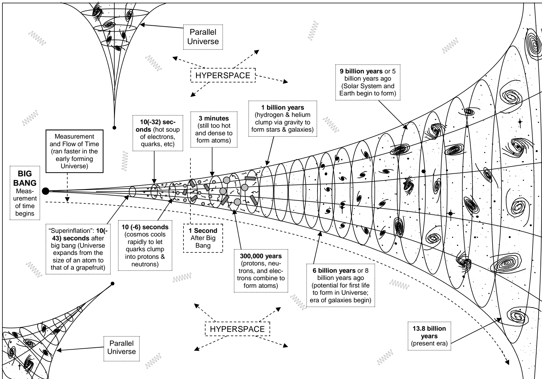
Figure 1.1: BIG BANG (Expansion of Universe)
